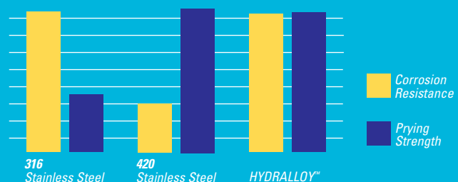
Compare HYDRALLOY™ to other stainless steel alloys
